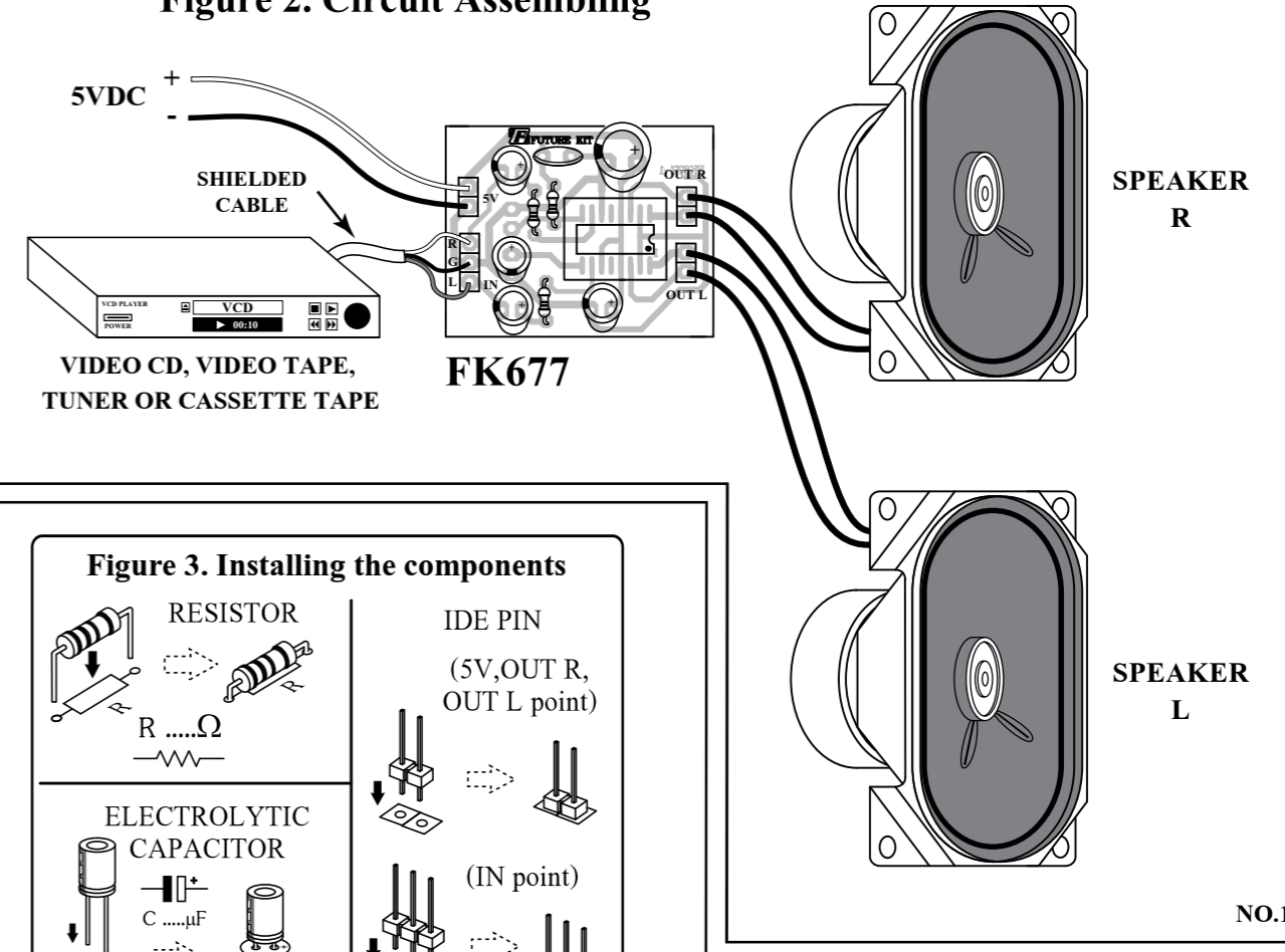
Figure 2. Circuit Assembling
