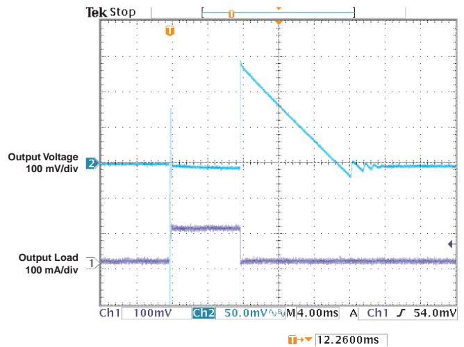
LOAD TRANSIENT RESPONSE vs TIME
